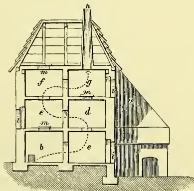
Condensing Chamber.
