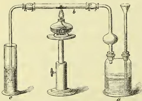
Apparatus for reducing tersulphuret of antimony.
