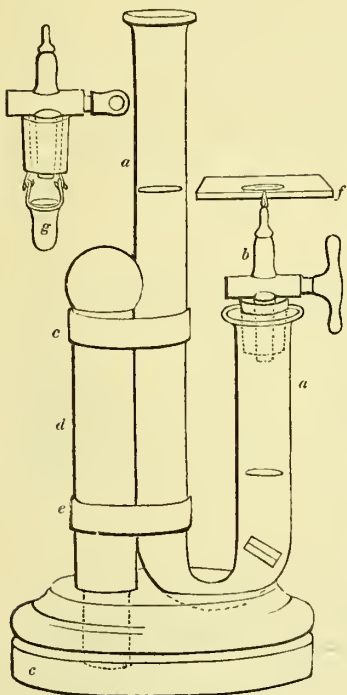
Marsh's Apparatus.
