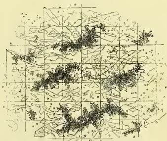
Microscopic appearance of commercial (i. e. impure) precipitated sulphur, shewing the crystals of sulphate of lime (selenite).
