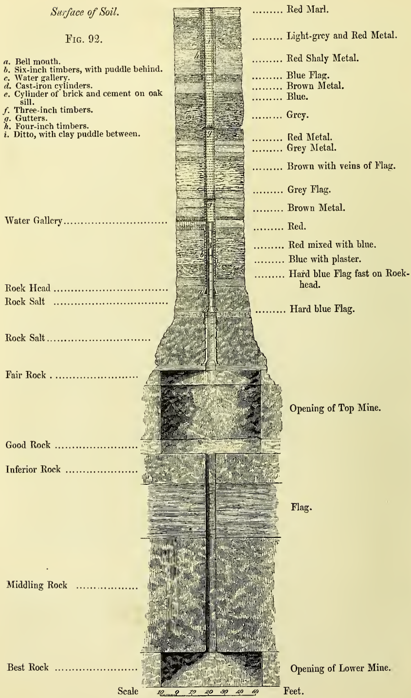
Section of the Wharton Salt Mine, on the River Weaver, Cheshire.
